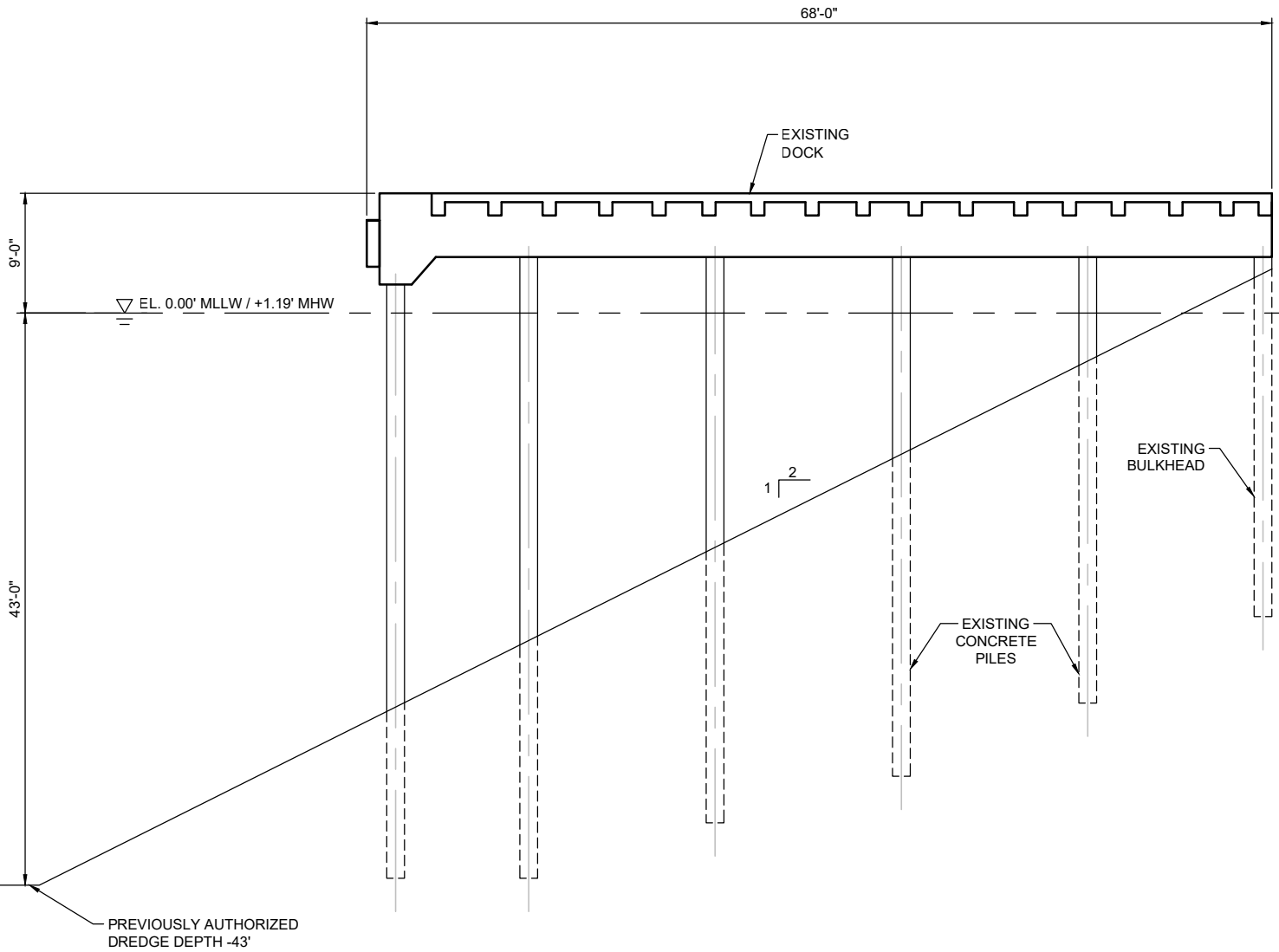
A 2 EXISTING CONDITION SCALE: 1"=150'
